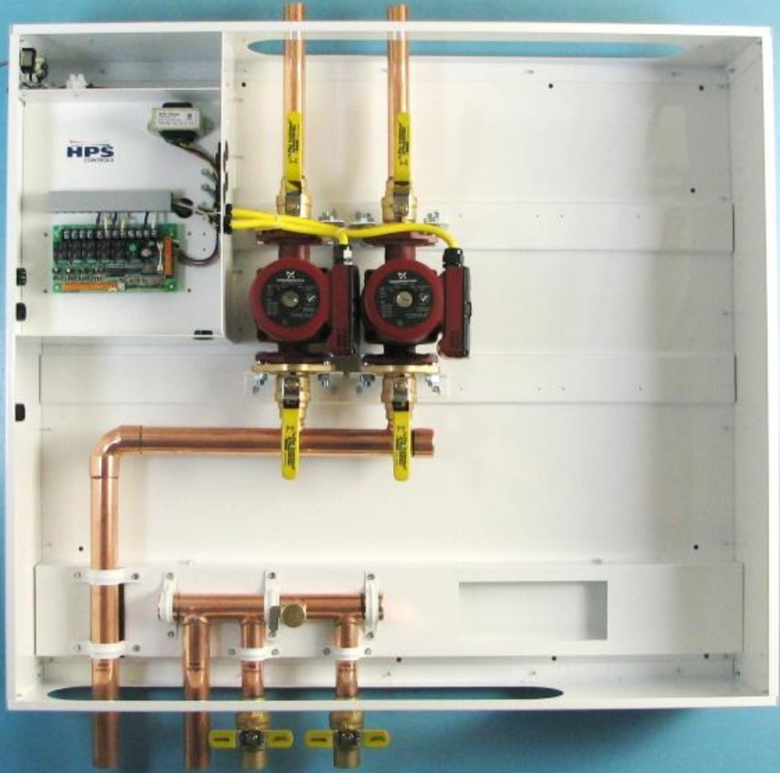
HFS-2 [High Temp 2 Zone Flange Pump Control Station]
